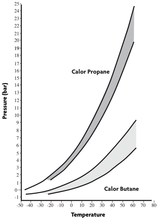
Vapour Pressures of Calor Butane and Calor Propane
